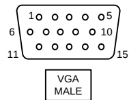
Front (mating) view
