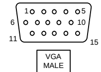
Front (mating) view
